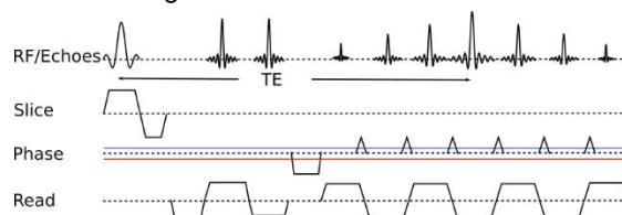
Fig. 1: Basic pulse sequence used in this study. A gradient offset (blue) is used during the entire slice to compensate a linear field inhomogeneity in the phase encoding direction (red). For a field inhomogeneity in the frequency encoding direction, a gradient offset in the readout direction would be required. The initial echoes are used for phase correction.
