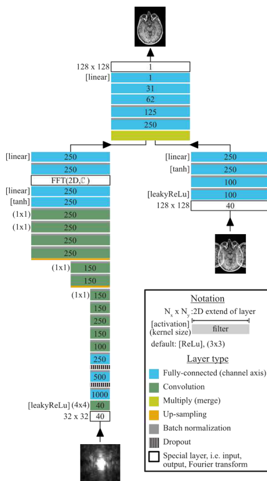
Fig. 1: Architecture of SMSnet. The 20-channel complex valued input data are split into their real and imaginary components which are then concatenated along the channel dimension resulting in 40 input channels. In the left branch, termed coil sensitivity path (CoS), features similar to coil sensitivities are derived from reduced k-space data (size: 32x32x40). These are then merged by element-wise multiplication with the input image data (size: 128x128x40) after passing the right branch, termed image-path, similar to the unfolding process in PI. The last section, termed merge-path, reduces the number of channels. The combined channels yielding a single magnitude image per slice at the output (size: 128x128) of SMSnet.
