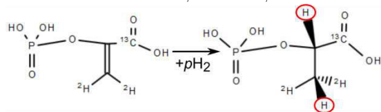
Fig. 2: Conversion of PEP (left) to PLAC (right) by catalytic hydrogenation. After hydrogenation, proton polarization (red circles) is transferred to ^{13}C by means of a spin order transfer sequence. The two protons, ^{13}C and ^{31}P were treated in the simulations.
